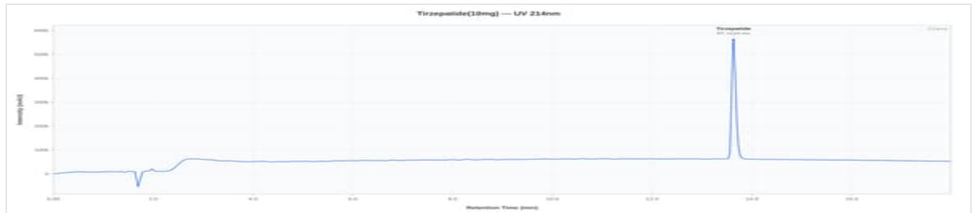
Tirzepatide 10mg - TR10-J19: UV Chromatogram
