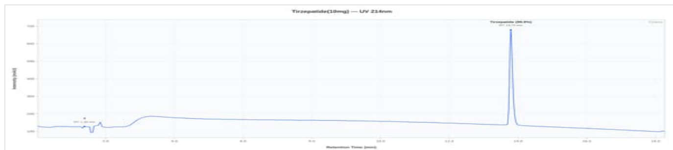
Tirzepatide 10mg - TR10-260806: UV Chromatogram
