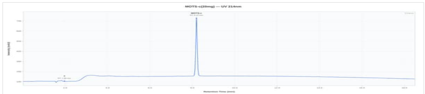
MOTS-C 20mg - MS20-L01: UV Chromatogram
