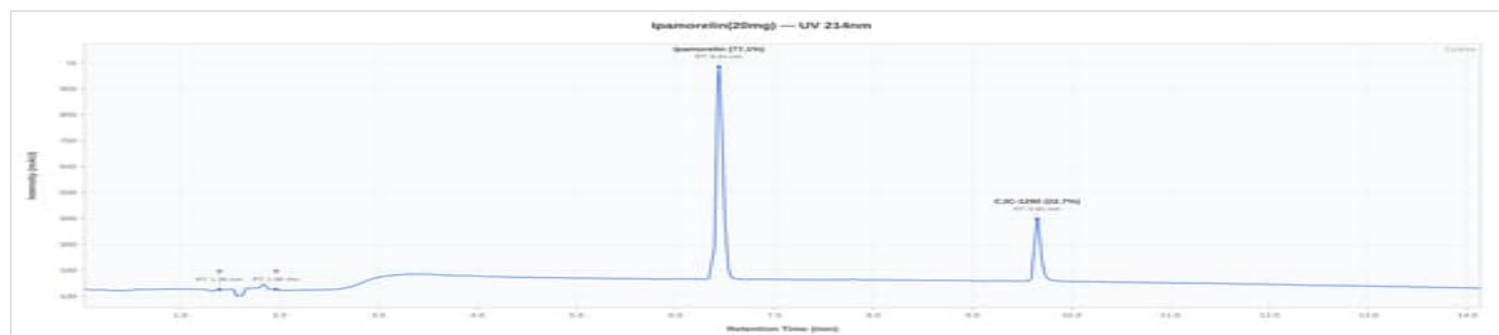
CJC-1295 / Ipamorelin 20mg - CP20-260806: UV Chromatogram
