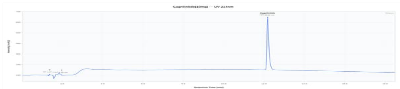
Cagrilintide 10mg - CGL10-L01: UV Chromatogram
